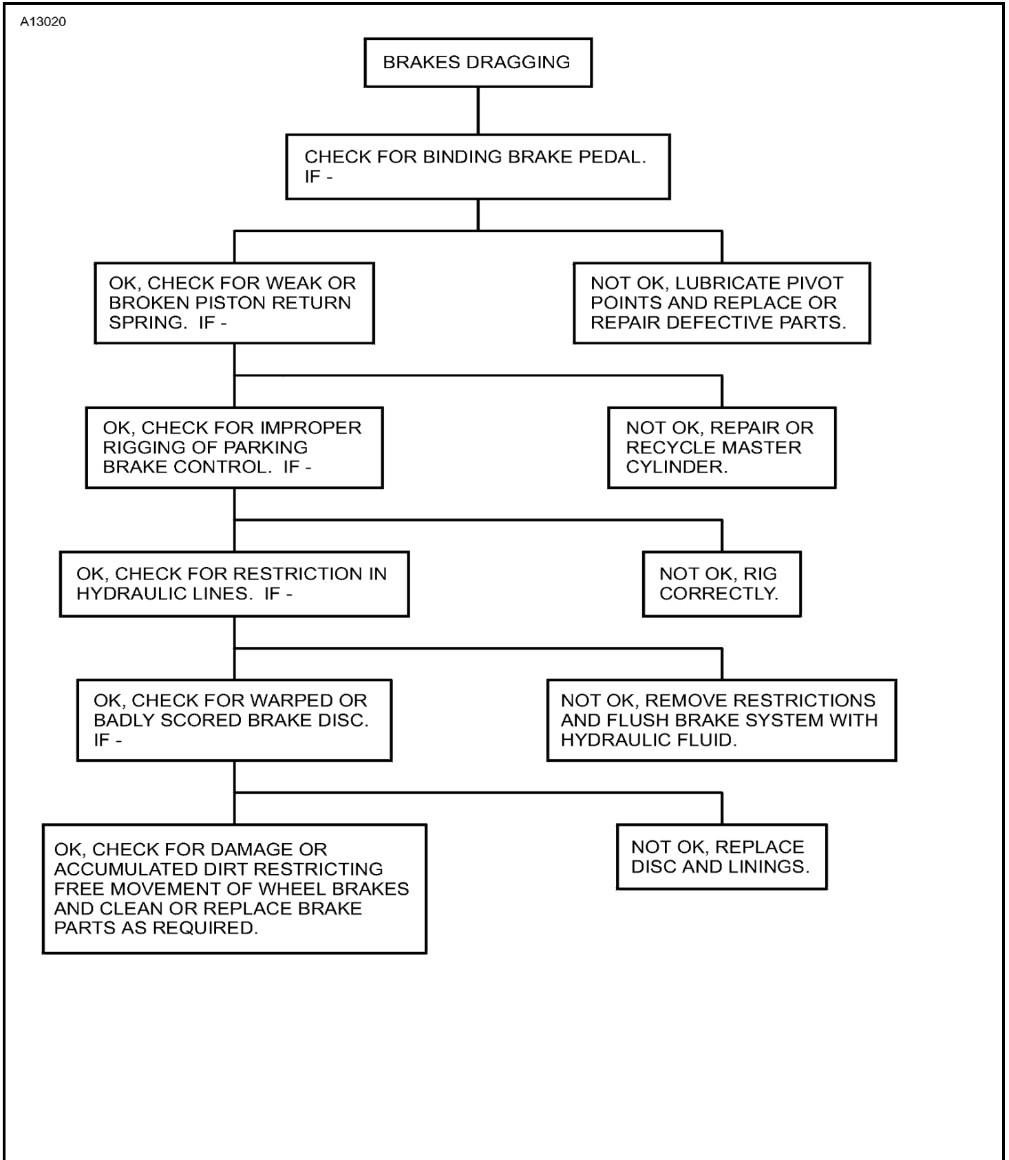
Figure 101 : Sheet 1 : Wheels and Brake Troubleshooting Chart
